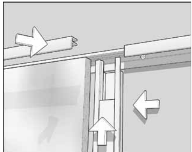
D2.4 Vertical CP-7 @ CP-280 Edge Trim Notch CP-7 to clear CP-280 flange
