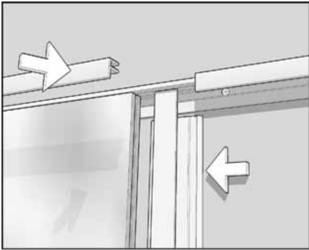
D2.1 Vertical CP-3 @ CP-280 Edge Trim Notch CP-3 to clear CP-280 flange
