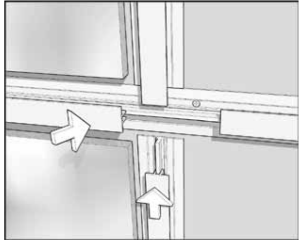
D5.2 Horizontal CP-4 @ Vertical CP-4 Butt vert. CP-4 retainer to horiz. CP-4 flange
