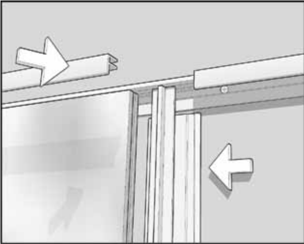
D2.3 Vertical CP-6 @ CP-280 Edge Trim Notch CP-6 to clear CP-280 flange
